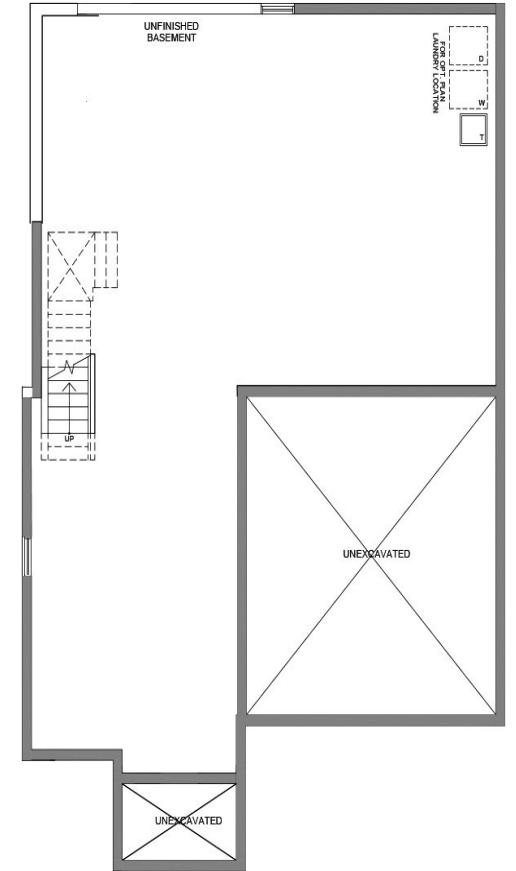
BASEMENT ELEVATION 1
